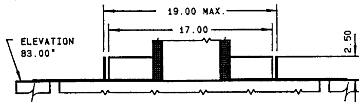
SEC. A-A FRONT VIEW, SUPPORT BRIDGE
