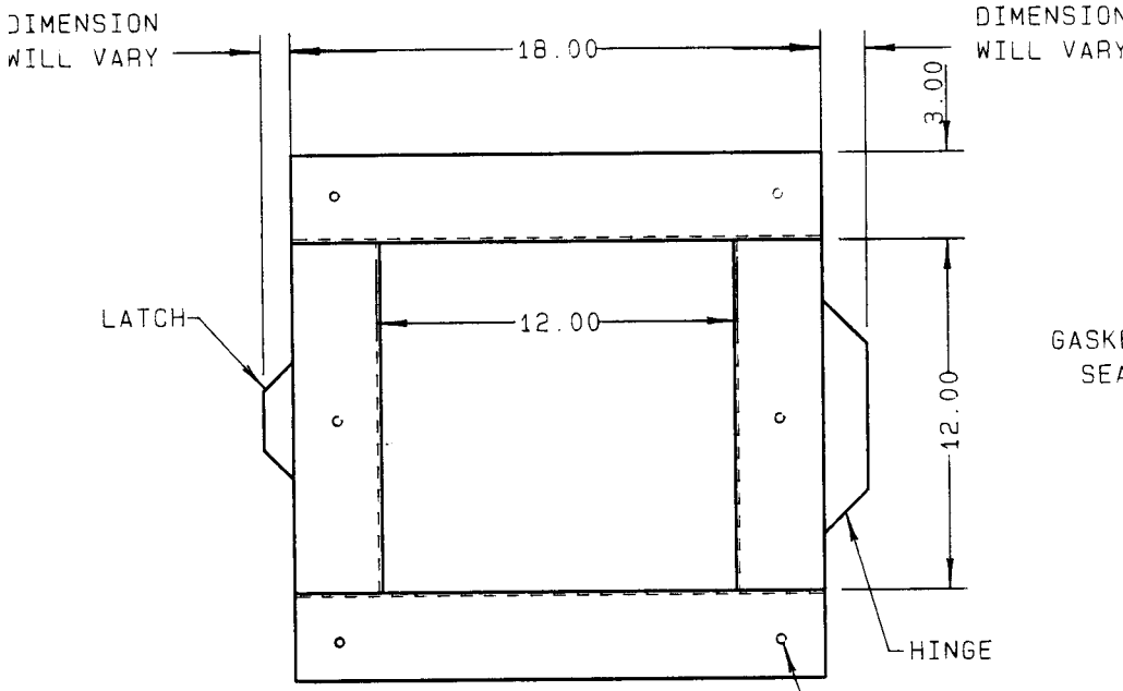
FIREBOX FRAME FRONT VIEW WITHOUT DOOR
