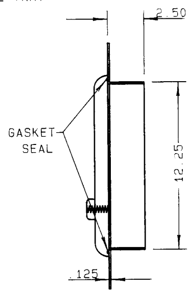
SIDE VIEW WITH DOOR
